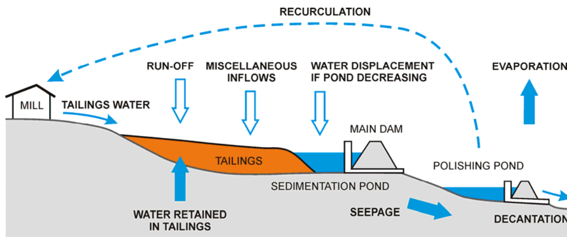
Figure 1: hydrological cycle of a TDF
