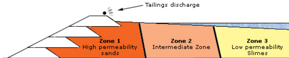
Figure 3: Tailings segregation zones
