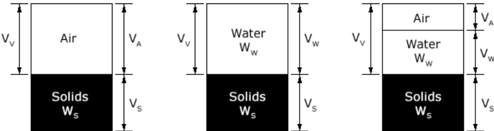
Figure 2: Water and air content in a soil [1]
